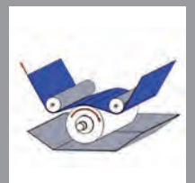
Kiss Coating
